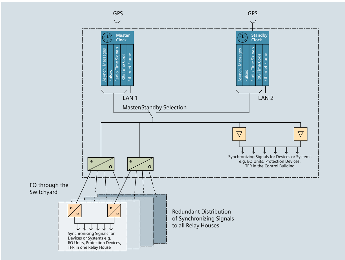
Fig. 4-8: Conceptual Overview of the Time Synchronisation
