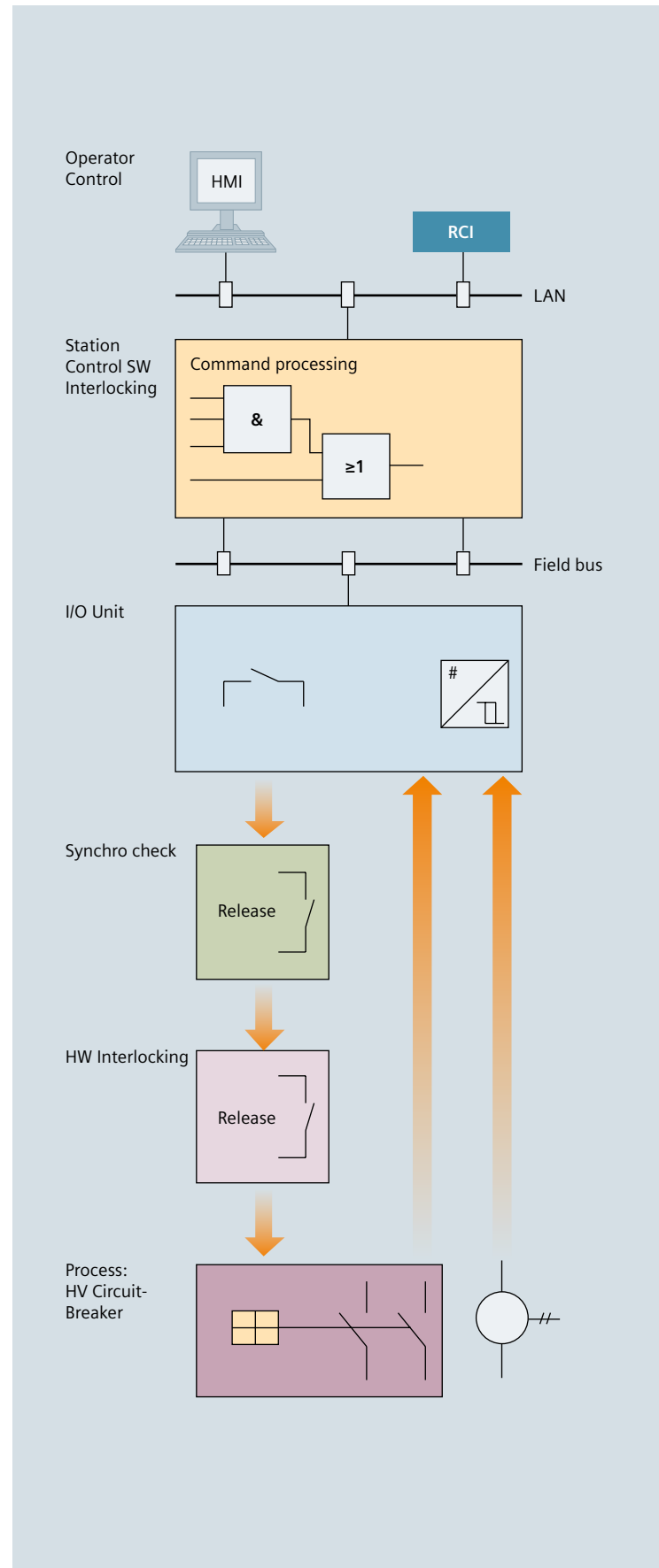
Fig. 4-14: Interlocking Philosophy
