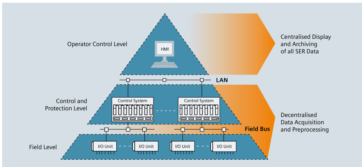
Figure 4-3: Decentralised SER Data Acquisition in Combination with Centralised Data Display
