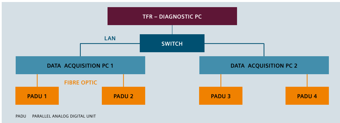
Fig. 4-6: Transient Fault Recorder Overview
