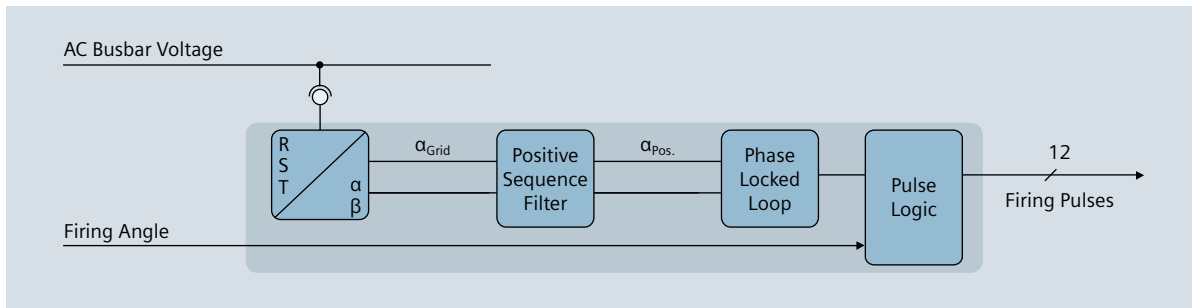
Fig. 4-16: High-Performance Firing Control System
