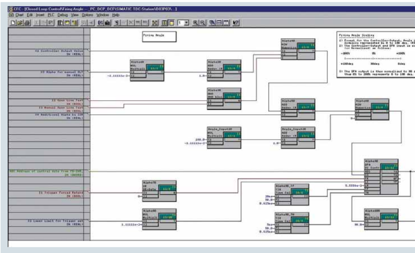
Figure 4-13: Graphical Engineering Tool CFC
