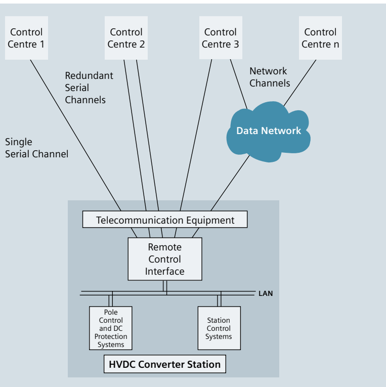
Fig. 4-7: Remote Control Interface (RCI) Embedded in the Communication Facilities
