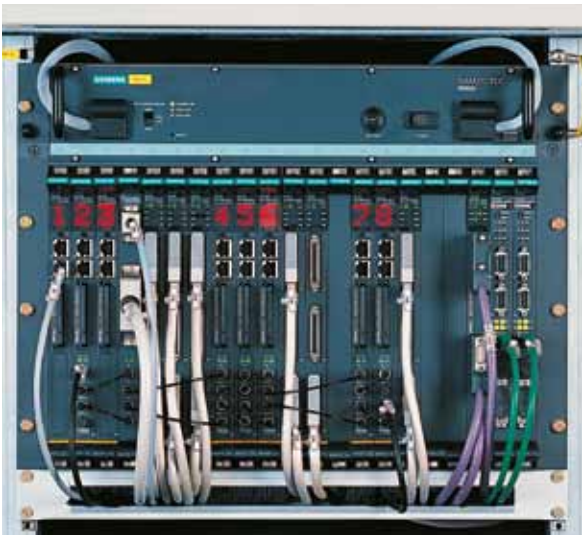
Figure 4-12: Standard SIMATIC TDC Control and Protection System
