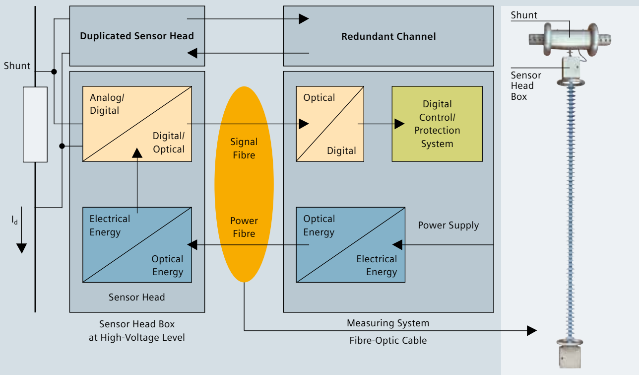
Fig. 4-21: Hybrid-Optical DC Current Measuring
