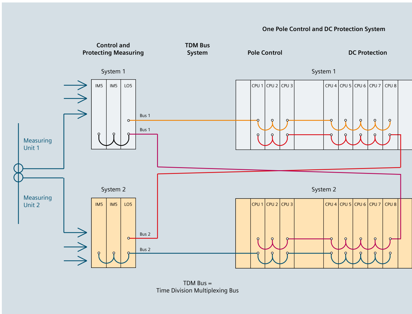
Fig. 4-20: Cross-Redundant TDM Bus
