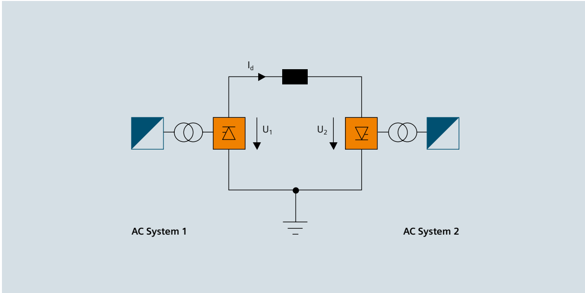
Fig. 3-1: Simplified HVDC System Diagram
