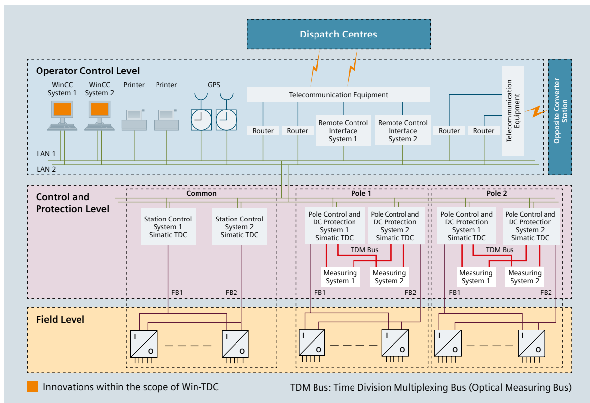
Fig. 4-1: Control and Protection Hierarchy (one Converter Station)
