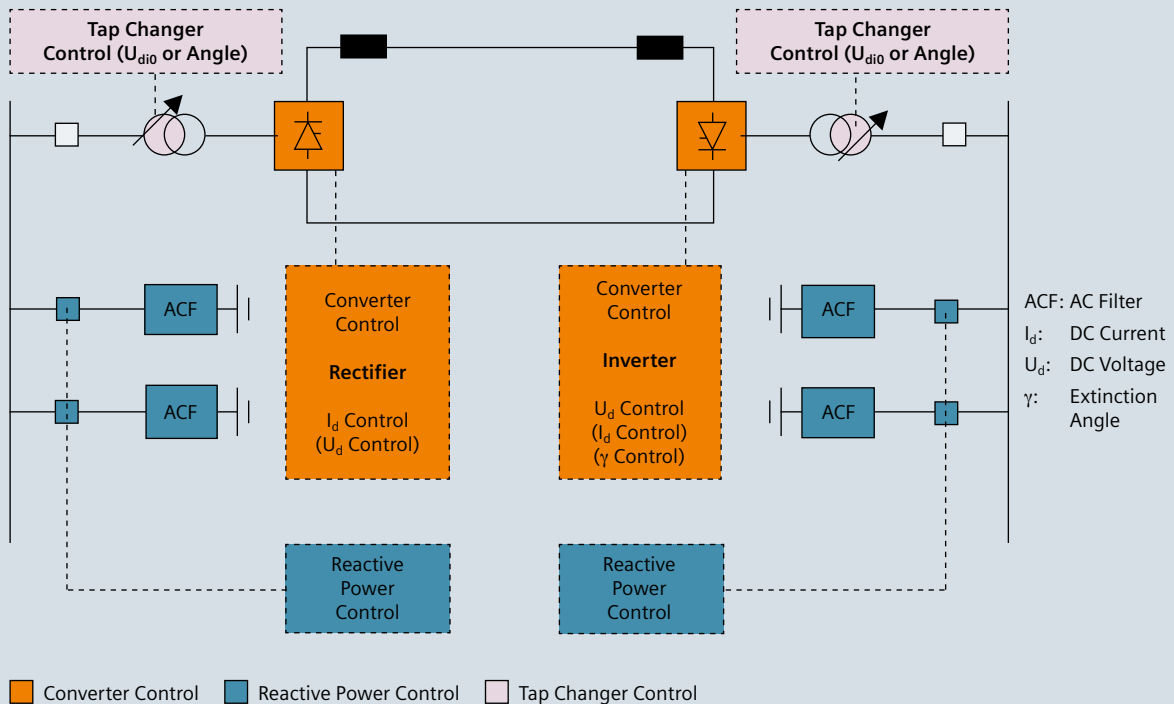
Fig. 3-3: Overview Control Functions
