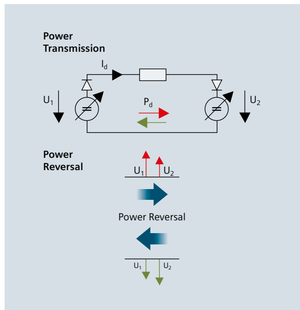
Fig. 3-2: Change of Power Direction (Power Reversal)
