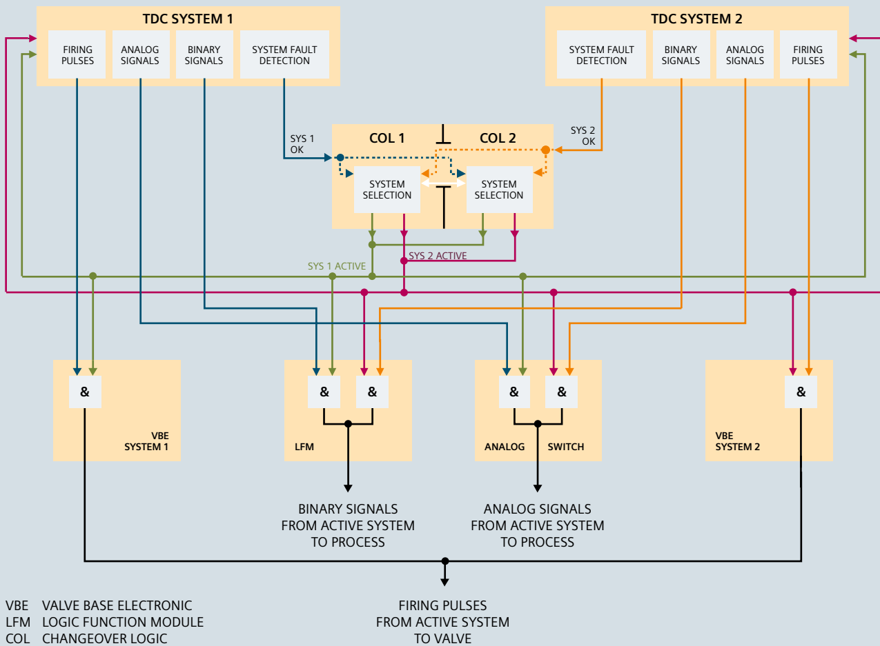
Fig. 4-19: Principle of Redundancy Management
