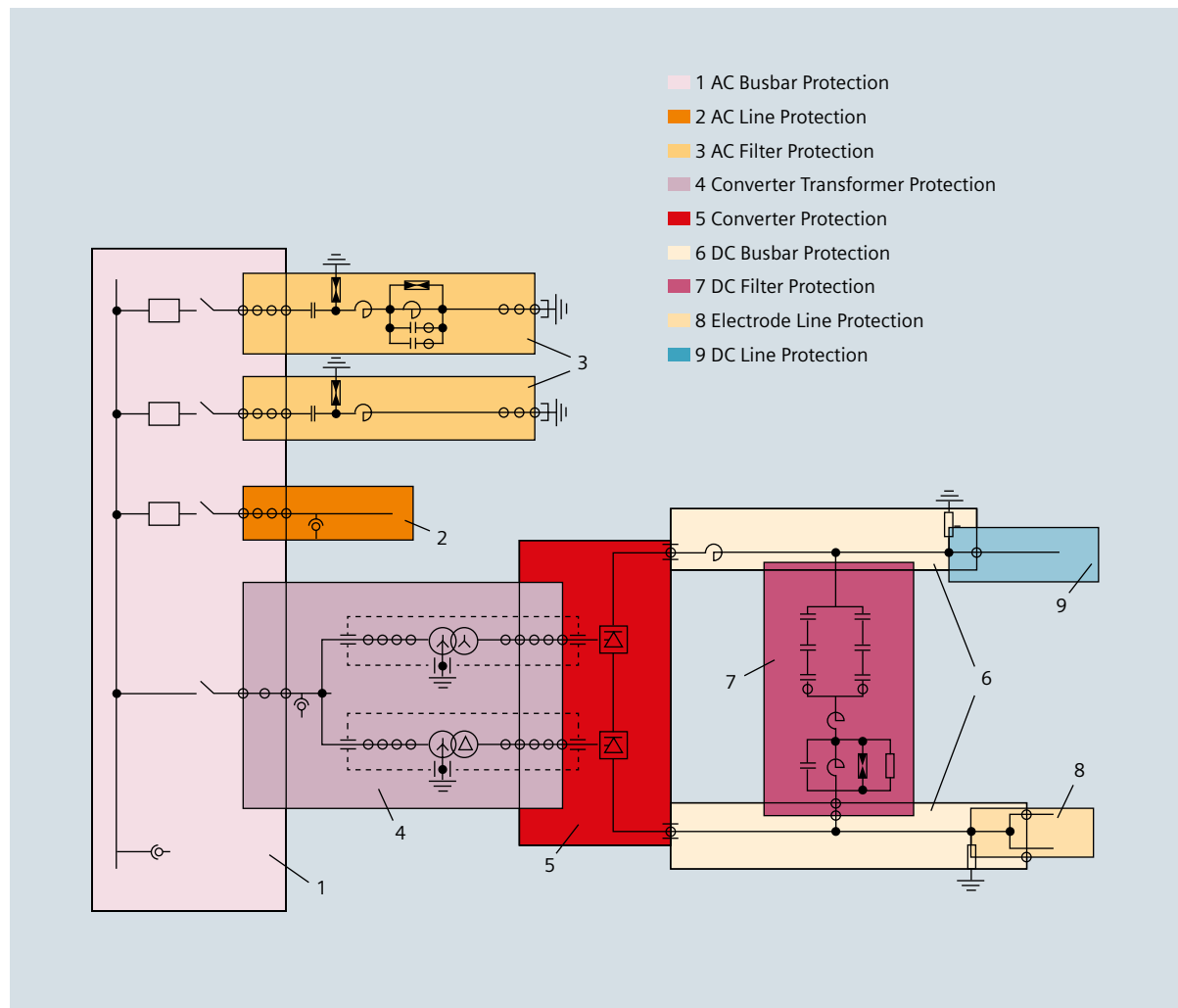
Fig. 4-17: Protection Zones for an HVDC Long-Distance Transmission Scheme
