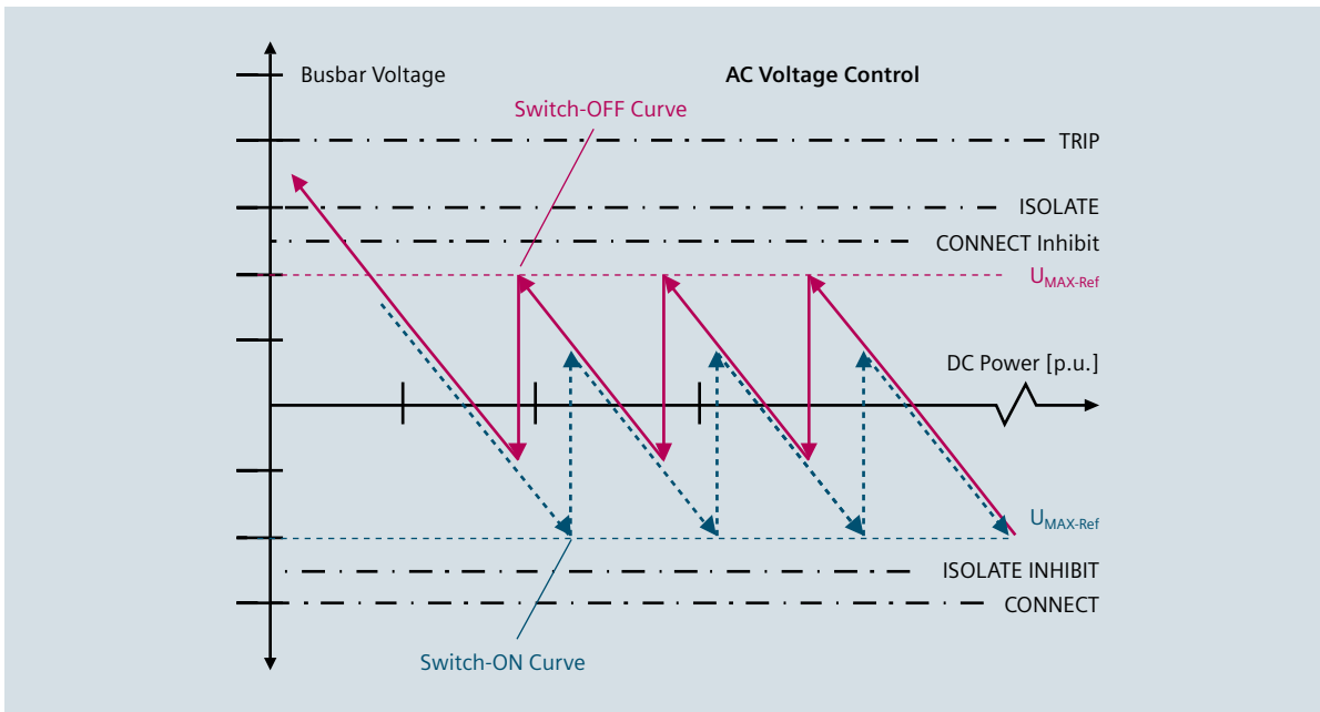
Fig. 4-15: Reactive Power – and AC Voltage Limitation Control
