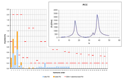
Figure 3: Harmonic spectrum at PCC
