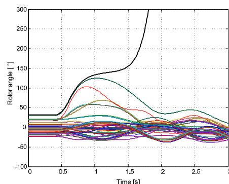
Figure 4: Transient stability after severe fault, a generator becomes unstable and is separated from the synchronous group
