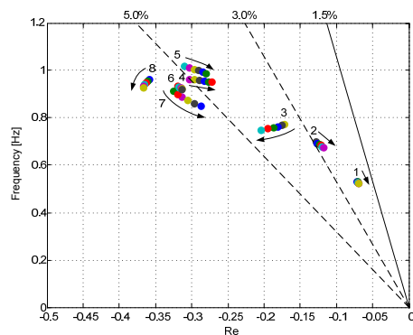
Figure 3: Presentation of system oscillation modes on complex plane with regard to variations in load or network topology alternations
