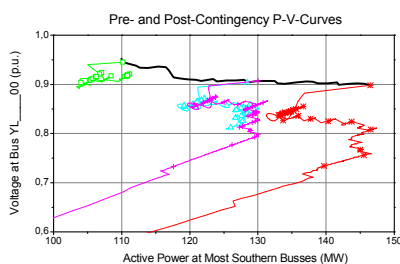
Figure 2: P-V curves from four different working points (red and magenta curve: voltage collapse)
