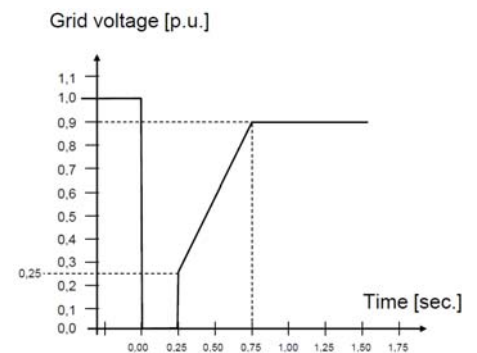
Figure 2: Example of a fault ride-through requirement curve
