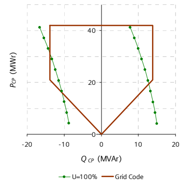
Figure 1: Example of reactive power capability curves
