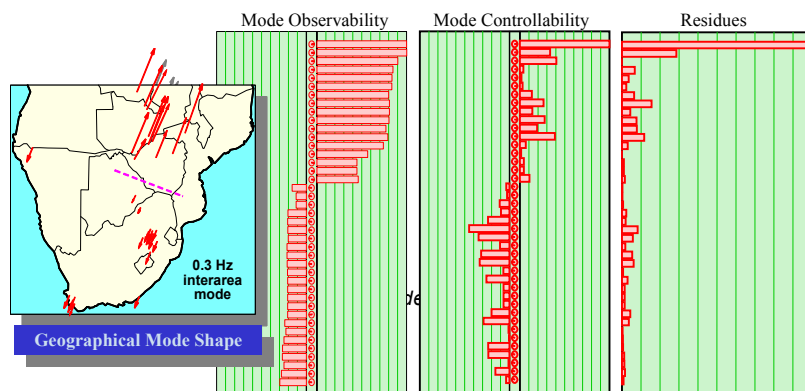
Figure 4: Eigenvectors of an inter-area mode
