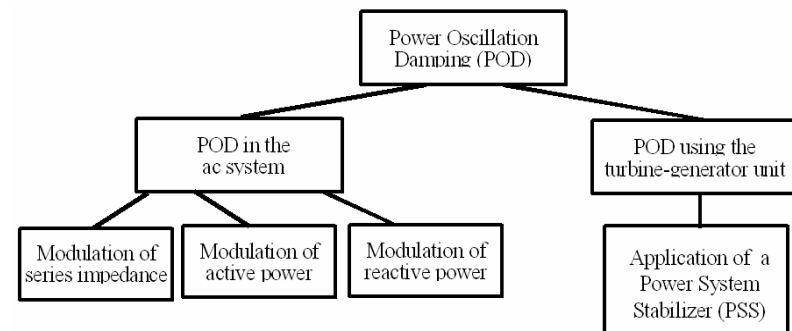
Figure 3: Strategies to damp power oscillations
