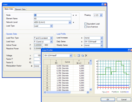
Figure 2: Load profile for a load
