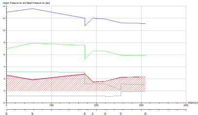
Figure 2: Profile curve for district heating
