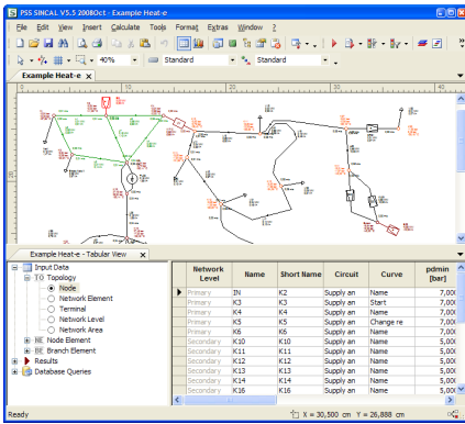
Figure 1: Steady-state simulation of a district-heating network
