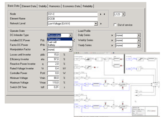
Figure 2: Specific modeling of distributed generation units
